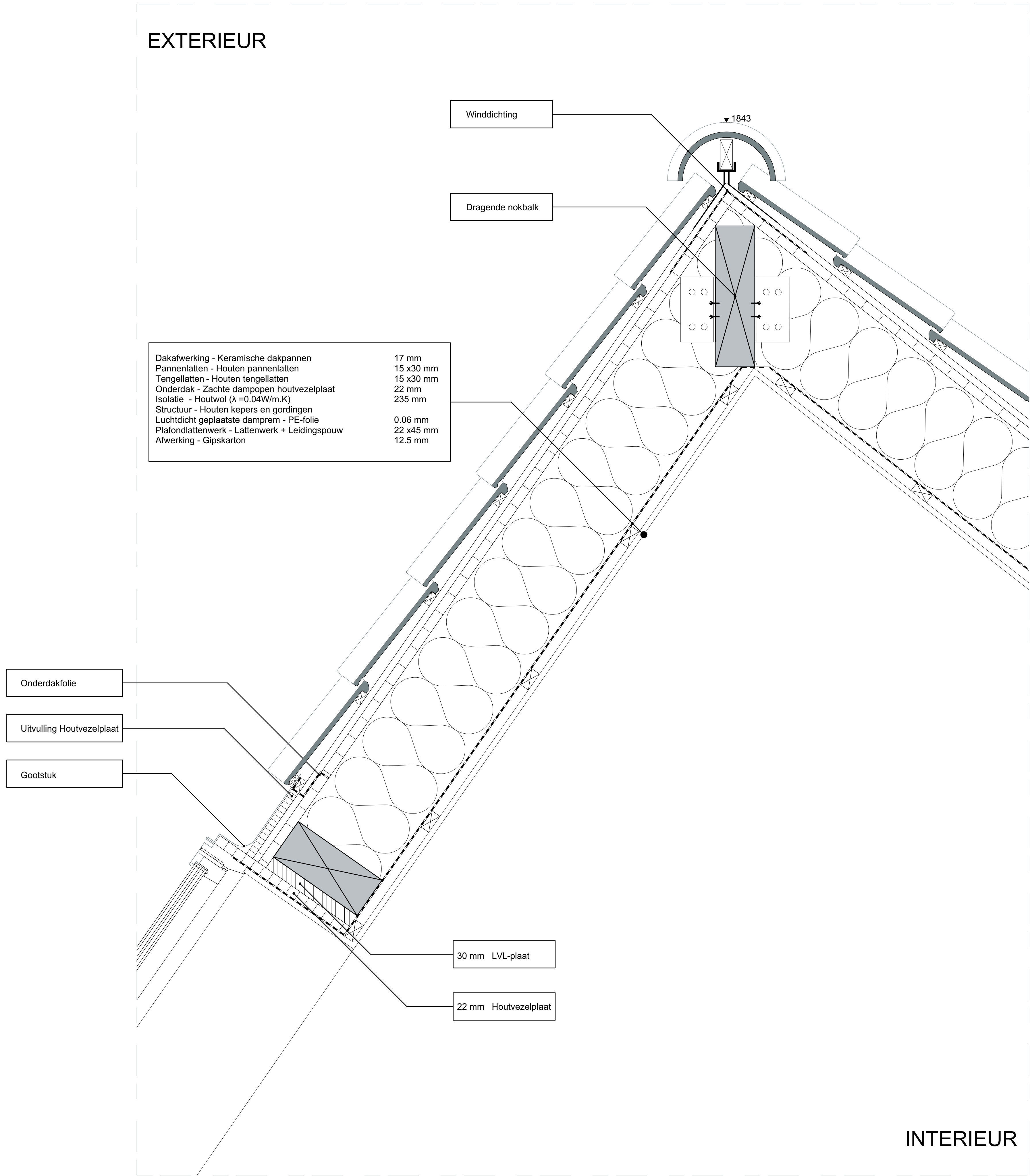
DETAIL 1 - 1/5
