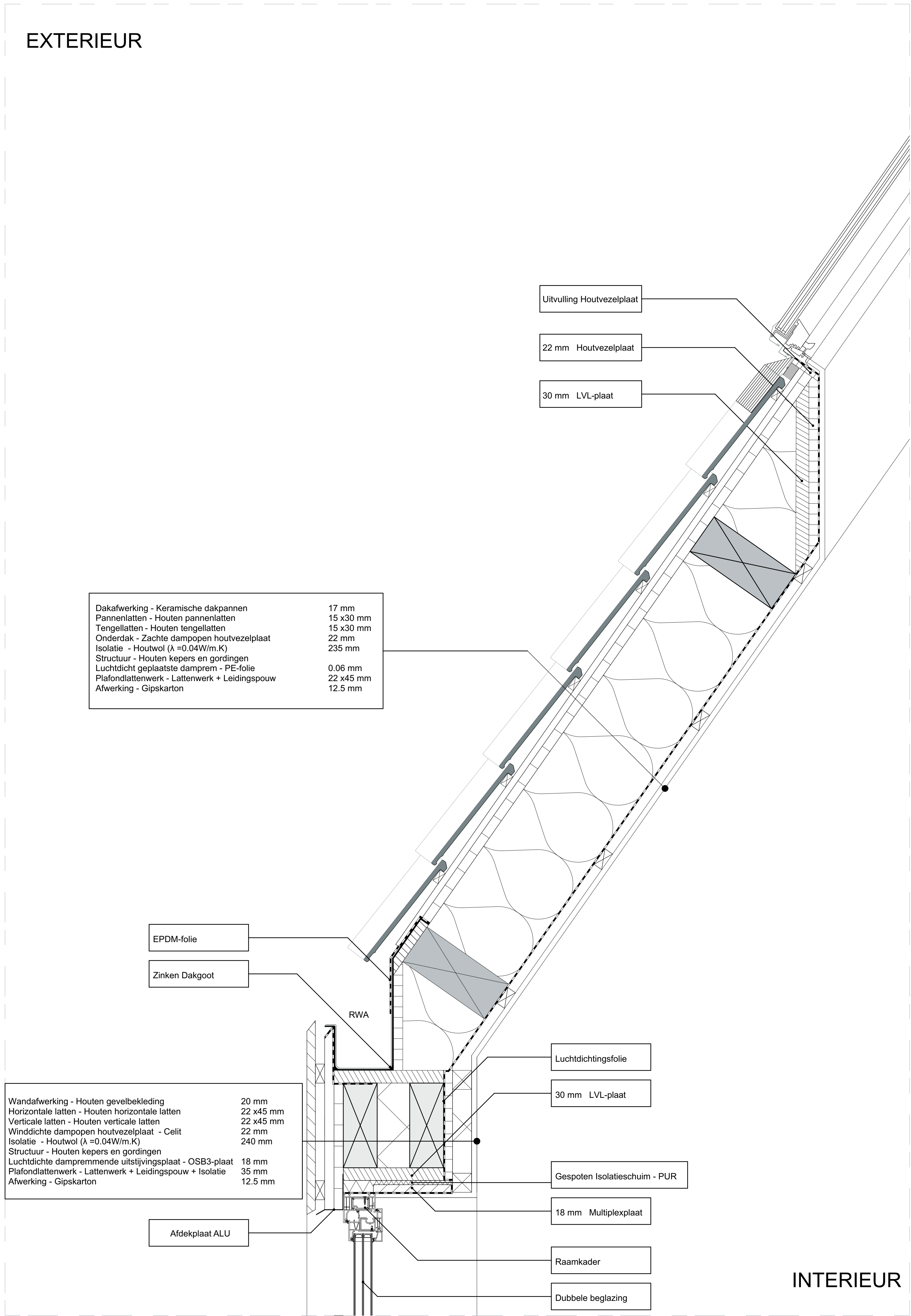
DETAIL 2 - 1/5
