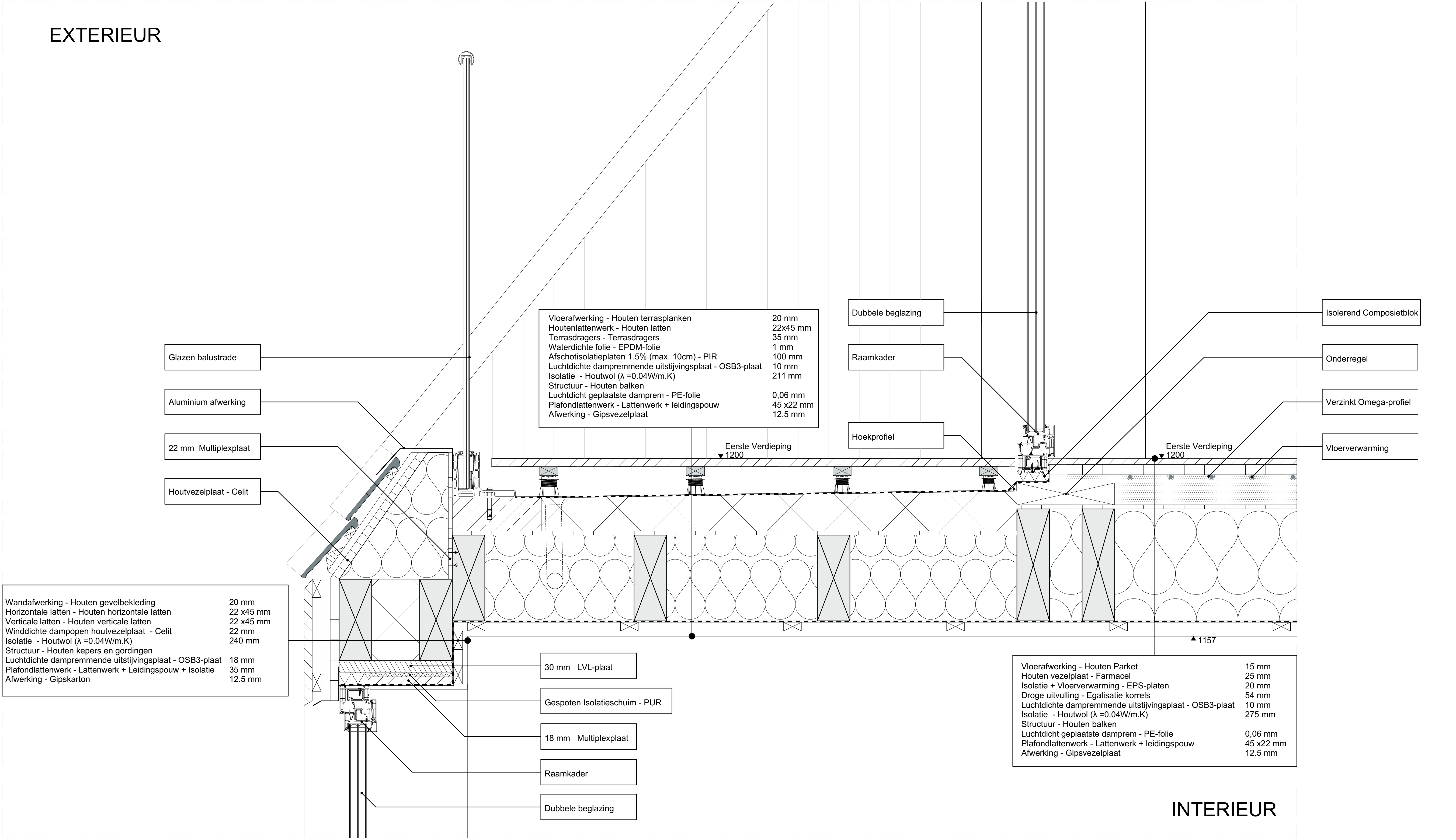
DETAIL 3 - 1/5
