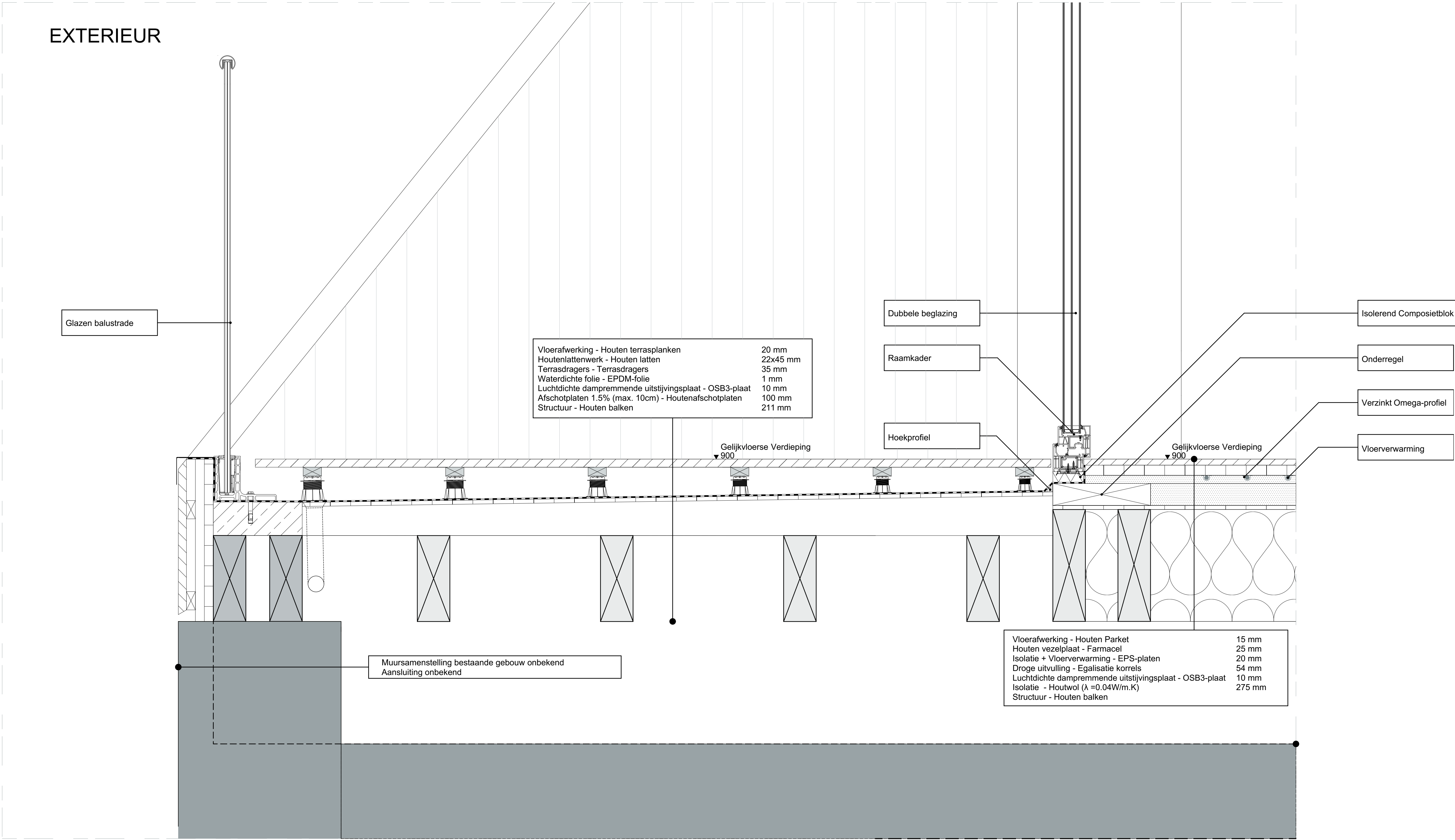
DETAIL 4 - 1/5
