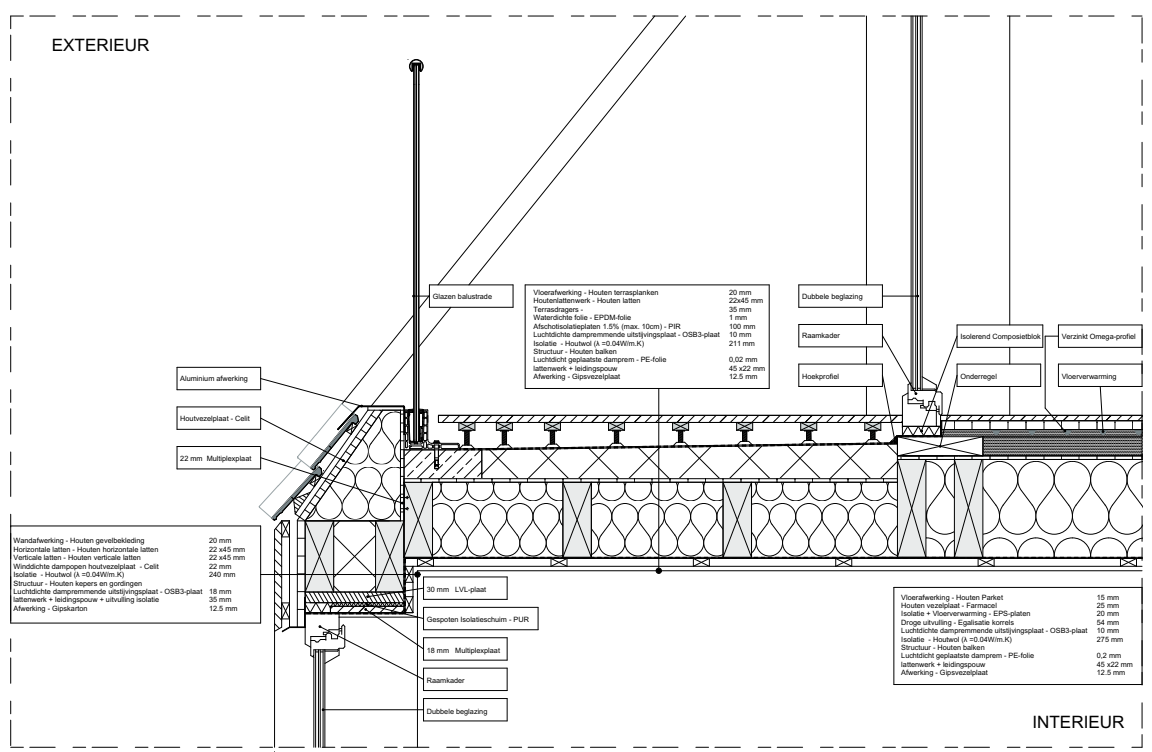
2D-Detail - BIM
